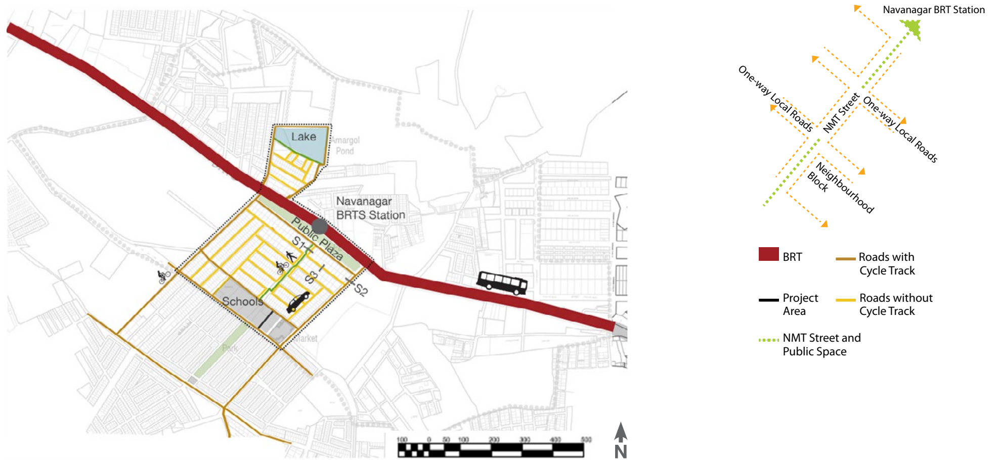
Figure 17 Plan showing NMT network in Navanagar in Hubli-Dharwad, India, Source: EMBARQ India
